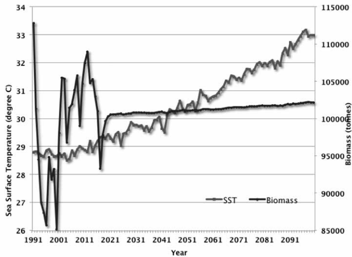
Plot of biomass estimates of lesser sardines and projected SST for the south Kerala region when the fishing effort is kept constant
