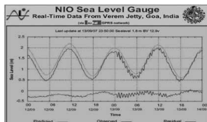
Internet-accessible, real-time graphical reporting of September 2007 Sumatra tsunami arrival at Goa through CSIR-NIO's cellular network of radar-based sea-level gauges.
