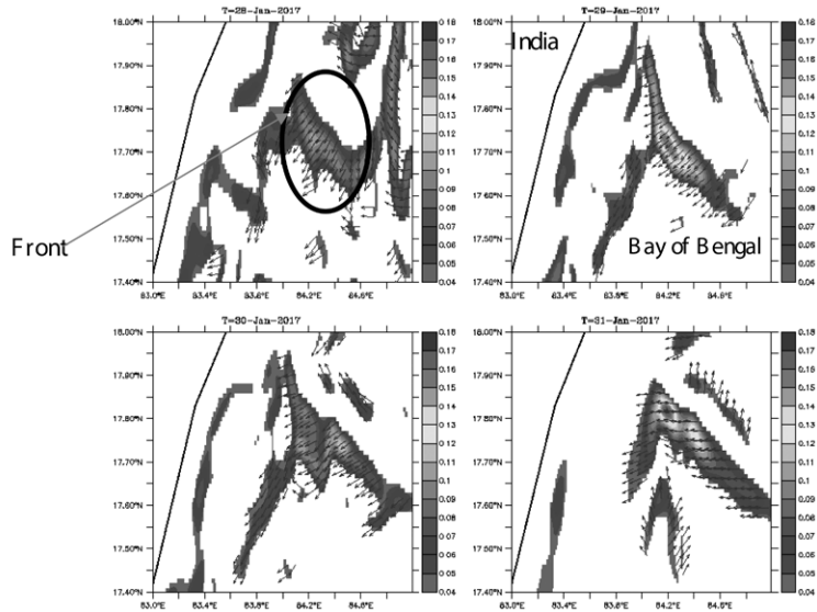
Figure 1: SST gradient and resultant vector for the period 28-Jan-2017 to 31-Jan-2017.
